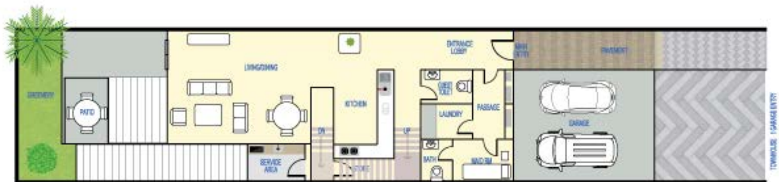
GROUND FLOOR PLAN | Floor Area 182.07 sq.m. (1,959 sq.ft.)
